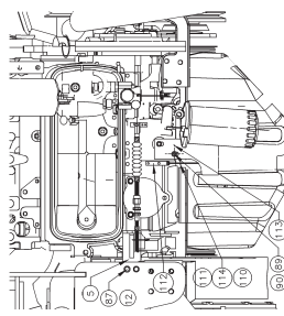
VIEW A ACCELERATOR CABLE INSTALLATION
